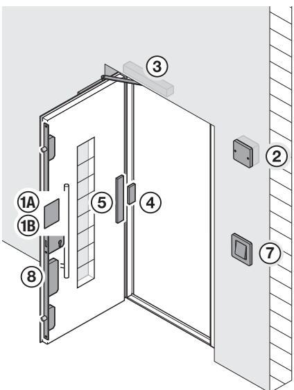
S5 Ecturn Scan / Code (KÜ)
